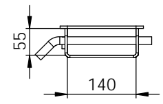
DETAIL B SCALE 2 : 5
